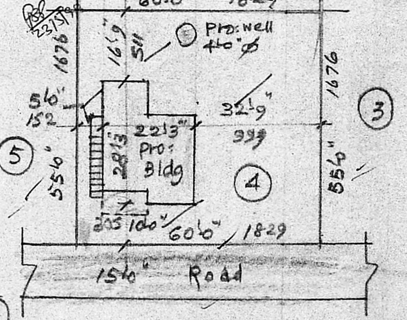
SITE PLAN Scale = (1" = 24') 1:300
